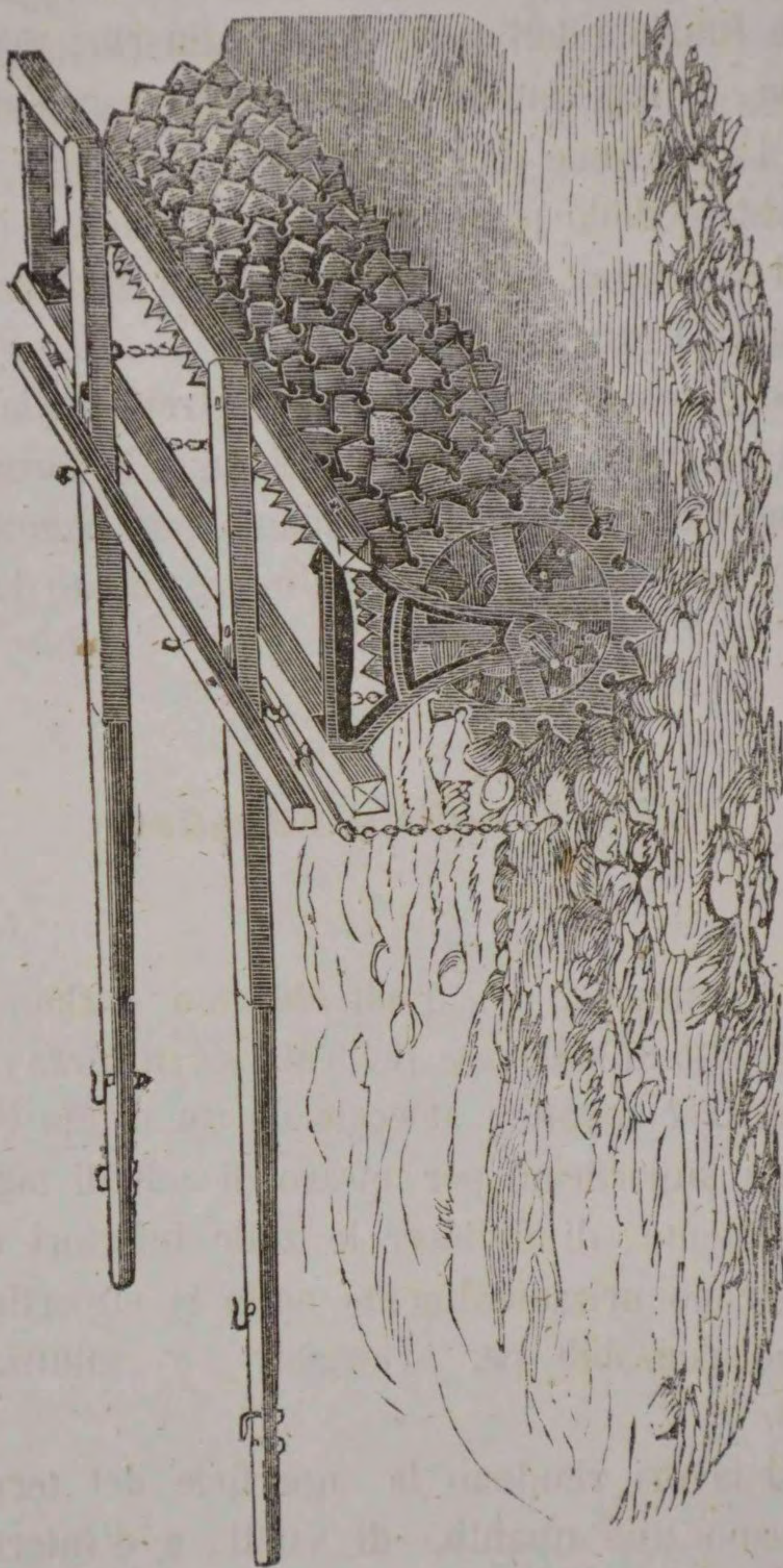
Fig. 47. — Rullo Crosskill.
